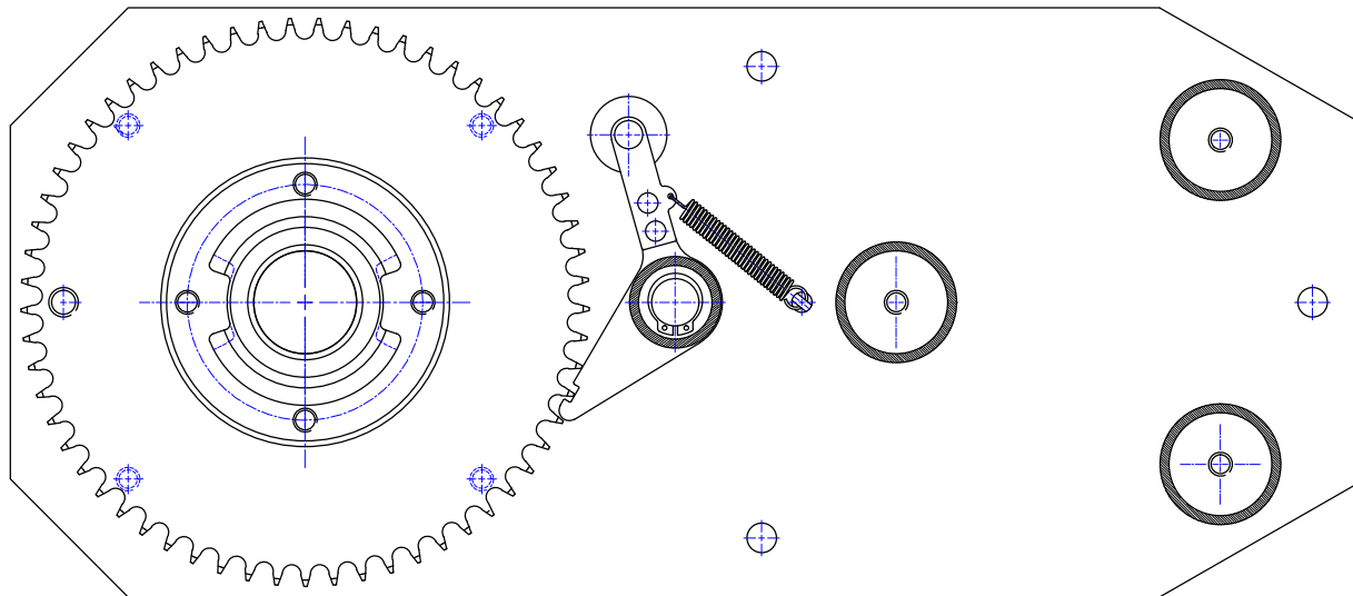
VIEW ON BRACKET PACK WITH CHAIN BREAK DEVICE ENGAGED AFTER CHAIN FAILURE.
