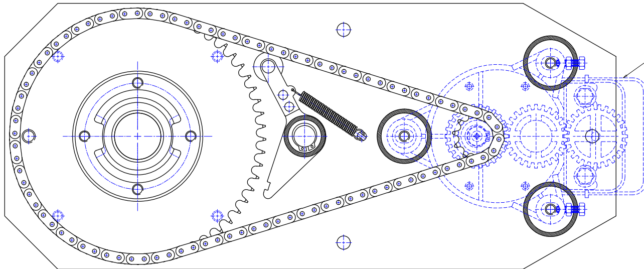
VIEW ON BRACKET PACK WITH CHAIN BREAK DEVICE IN NORMAL RUNNING POSITION
