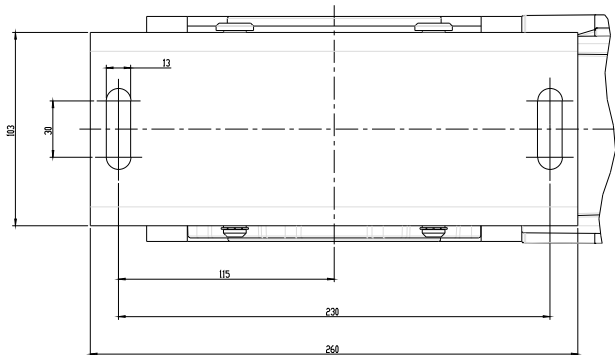
View X
