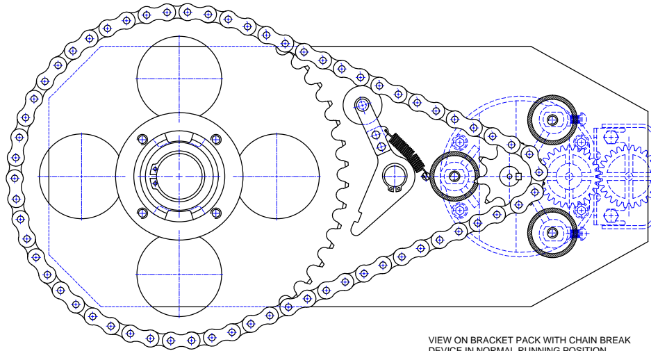
VIEW ON BRACKET PACK WITH CHAIN BREAK DEVICE IN NORMAL RUNNING POSITION
