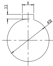
Bore Detail Scale 2:1
