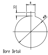
Bore Detail
